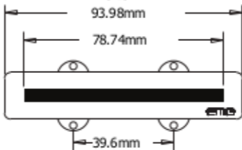
LONG J HOUSING (LJ)
